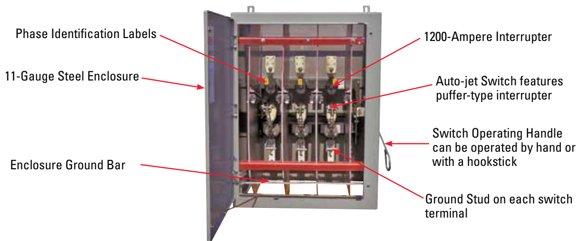
Interior view of wall-mounted switch to show Auto-jet® switch.
