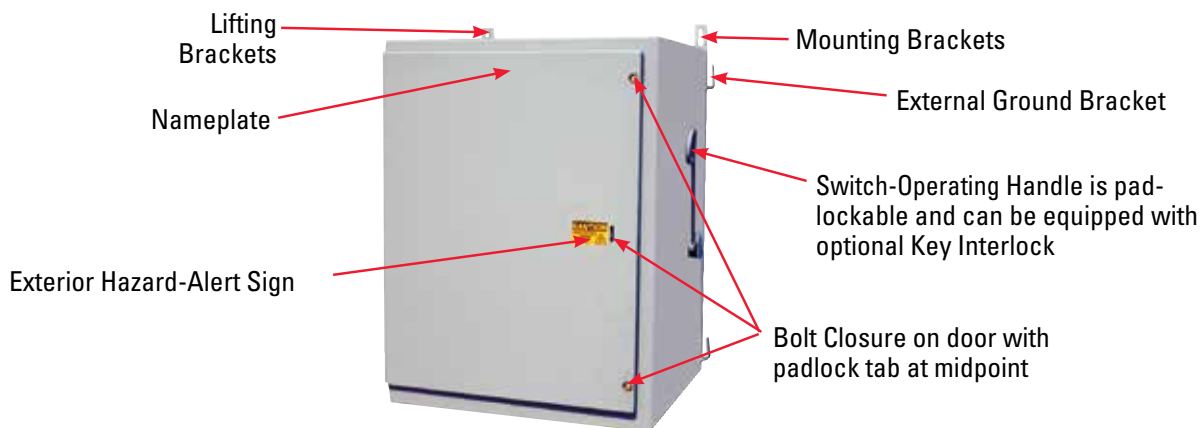
Exterior view of rugged Federal Pacific Wall-Mounted Switch Enclosure.
