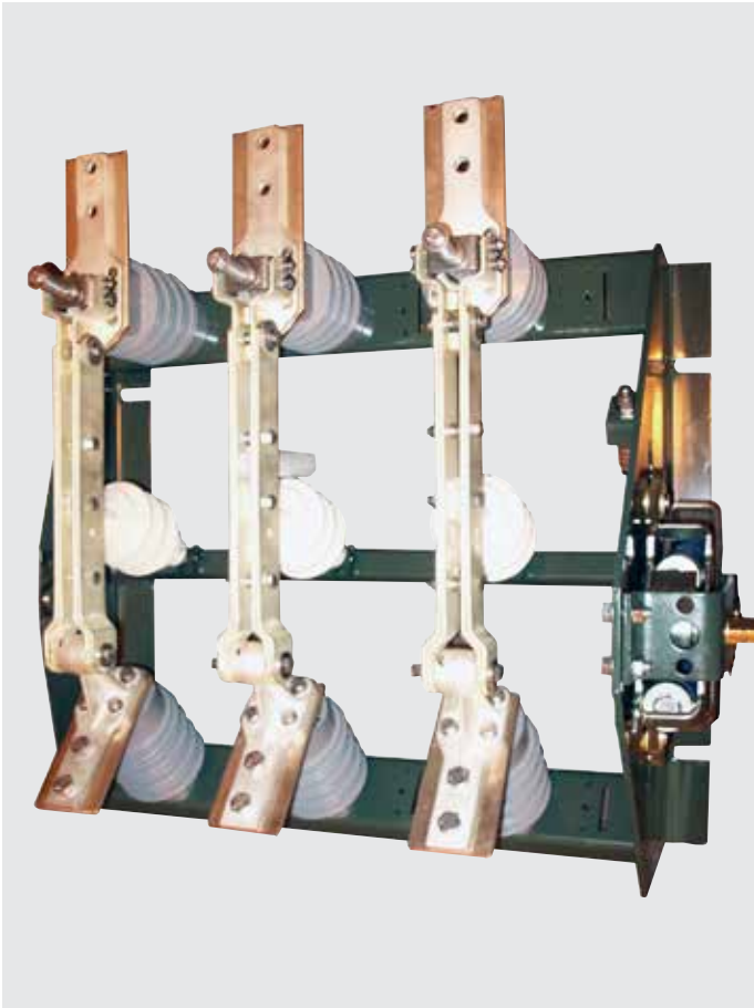
Pictured above are two views of the 1200-ampere switch showing the heavy blade structure and terminals — all silver plated.
