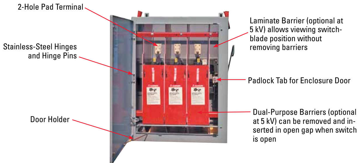
Interior view of wall-mounted switch to show barrier arrangement (barriers are optional at 5kV).
