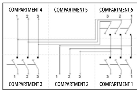
Drawing Number 37-0146-023 – Bus-Tie Configuration with two outgoing bus-only taps
