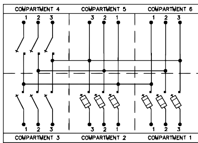
Drawing Number 37-0146-032E – Two incoming switches, two fused feeders and two bus-only feeders
